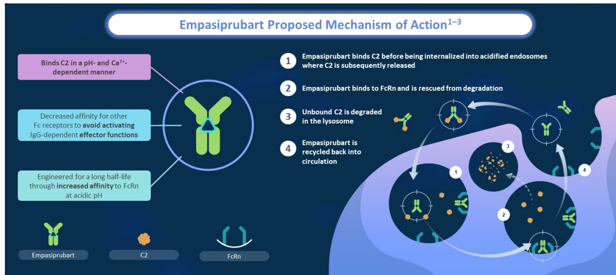
Figure 2: empasiprubarb mechanism of action. C2, complement component 2; FcRn, neonatal Fc receptor; IgG, immunoglobulin G.
